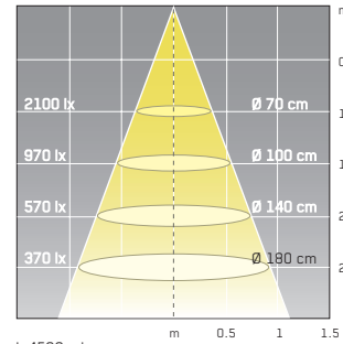
metal halide reflector, CDM-R 111, GX 8.5, 35W, 40°
