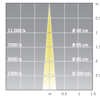
metal halide reflector, CDM-R 111, GX 8.5, 35W, 10°
