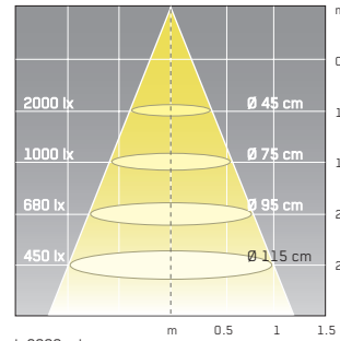
halogen reflector, Qr 111 - G53, 100W, 45°
