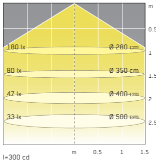
LED reflector, HALOLED - E27, 12W -warm white, 25°
