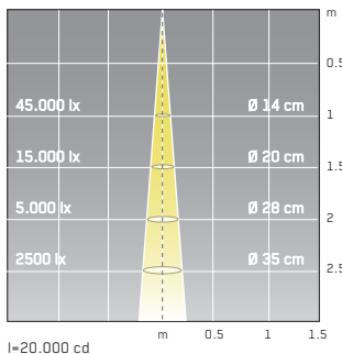
halogen reflector, Qr 111 - G53, 50W, 8°
