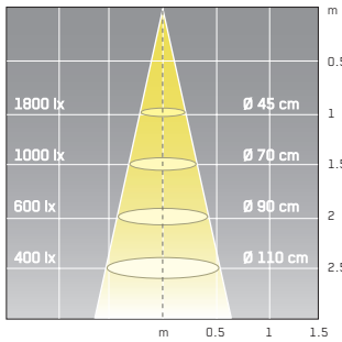
LED reflector, HALOLED - E27, 12W -warm white, 25°
