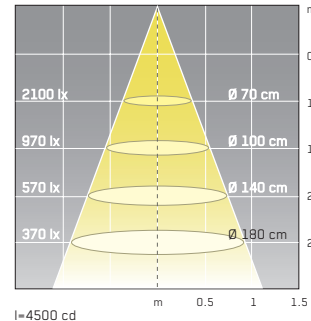
metal halide reflector, CDM-R 111, GX 8.5, 35W, 40°
