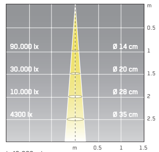
halogen reflector, Qr 111 - G53, 100W, 8°
