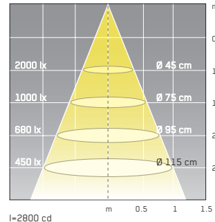
halogen reflector, Qr 111 - G53, 100W, 45°
