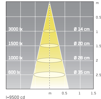
metal halide reflector, CDM-R 111, GX 8.5, 35W, 24°
