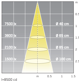
halogen reflector, Qr 111 - G53, 100W, 24°
