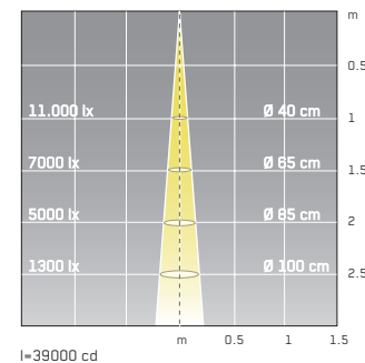
metal halide reflector, CDM-R 111, GX 8.5, 35W, 10°
