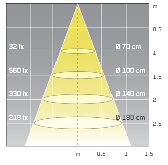
LED reflector, HALOLED - E27, 12W -warm white, 40°
