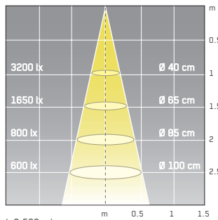
halogen reflector, Qr 111 - G53, 50W, 24°
