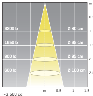
halogen reflector, Qr 111 - G53, 50W, 24°
