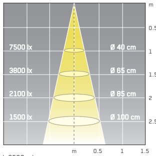
halogen reflector, Qr 111 - G53, 100W, 24°
