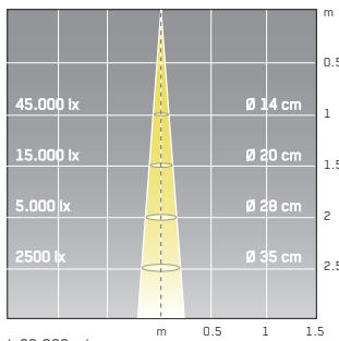
halogen reflector, Qr 111 - G53, 50W, 8°
